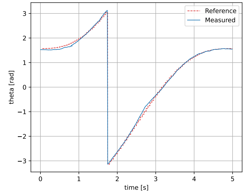
theta State
